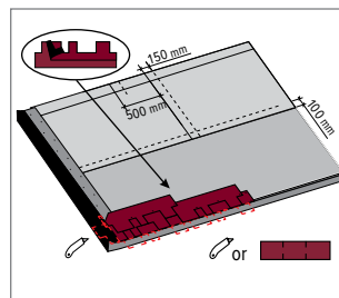
“accord” cutting pattern
