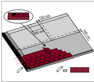
"bricks" cutting pattern
