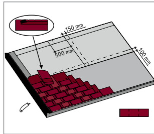
"continent" cutting pattern
