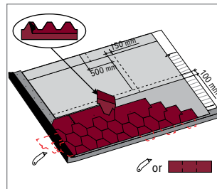
“sonata” cutting pattern
