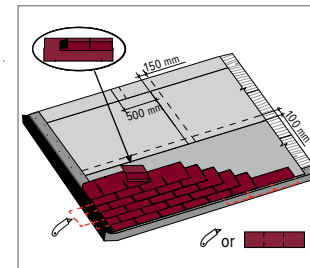
“trio”, “quattro” cutting pattern
