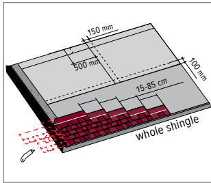
"castle" cutting pattern
