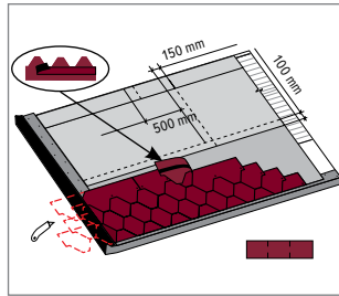
"western" cutting pattern
