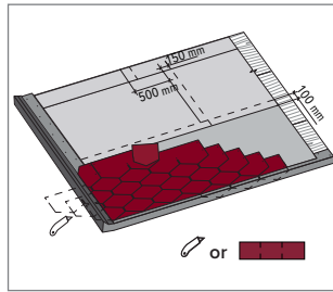
"delta" cutting pattern
