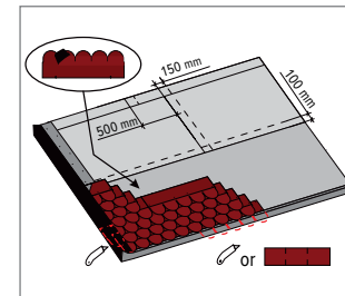
“beaver tail” or cutting pattern
