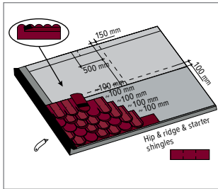
"atlantic" cutting pattern
